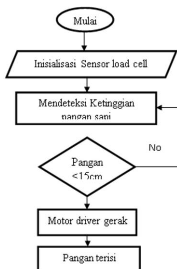
Gambar 2 Flowchart Sistem
