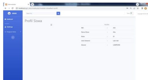
Gambar 6 Menu Profile
