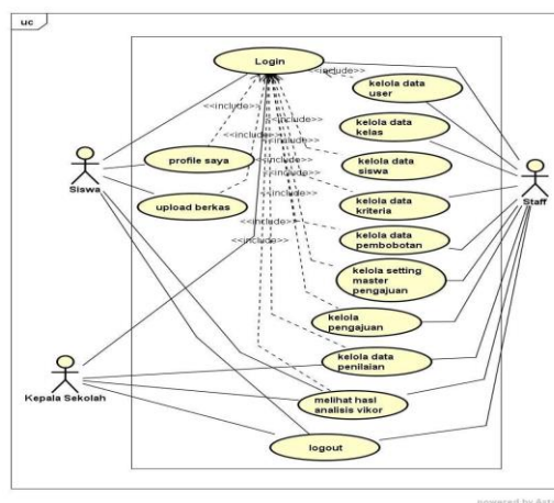
Gambar 3 Usecase Diagram
