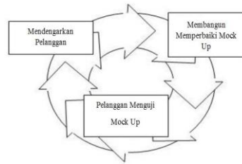
Gambar 1 Model Prototype .
