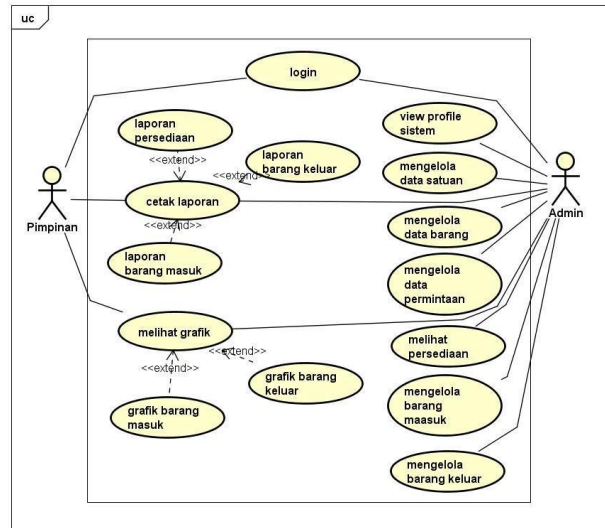
Gambar 2. Usecase Diagram
