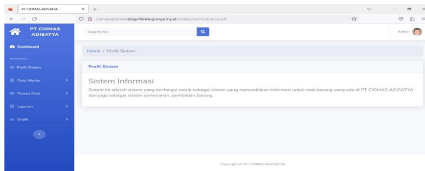
Gambar 6. Menu Profile
