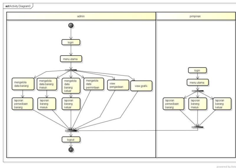
Gambar 3. Activity Diagram
