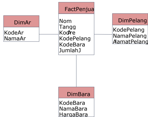
Gambar 2. Star Schema Data Warehouse
