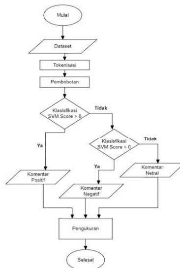
Gambar 3. Klasifikasi Support Vector Machine
