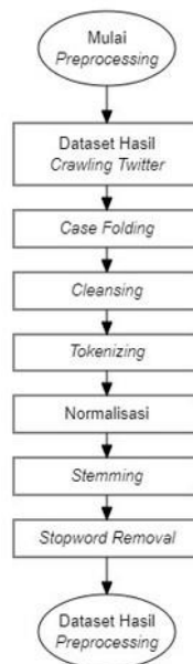
Gambar 2. Tahapan preprocessing
