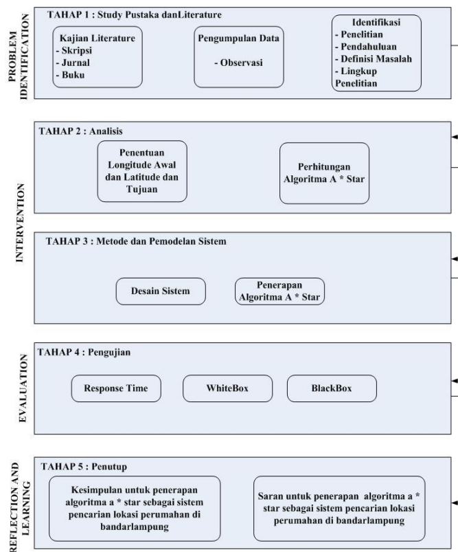
Gambar 1 Metode Penelitian
